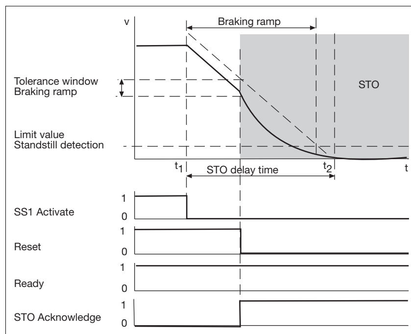
Fig. 4-3: Safety function SS1
