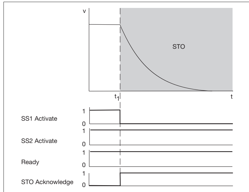
Fig. 4-2: Safety function STO
