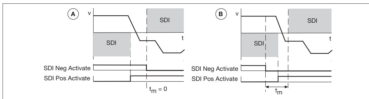
Fig. 4-11: Changing the direction of rotation
