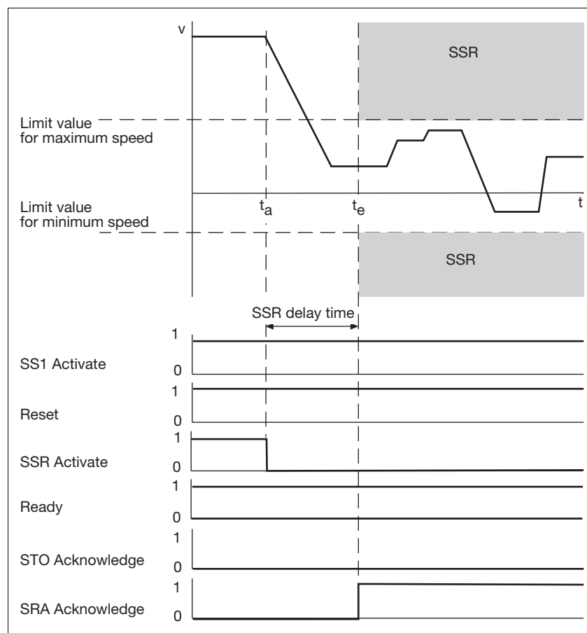
Fig. 4-8: Safety function SSR without tolerance range activated
