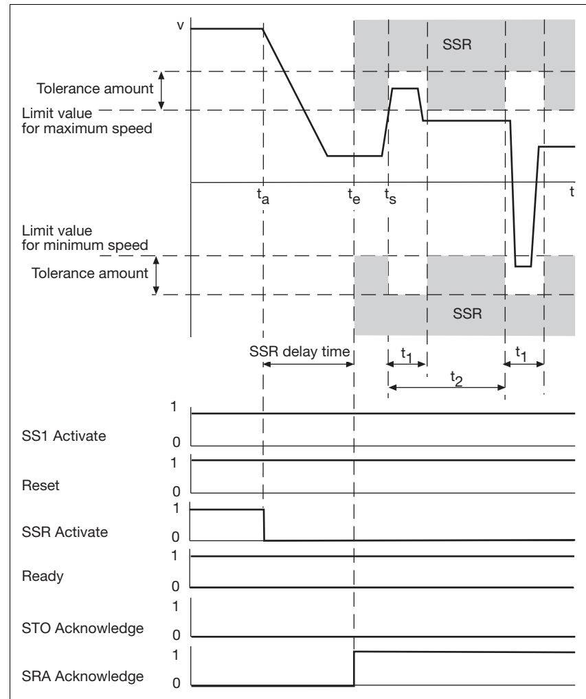
Fig. 4-9: Safety function SSR with tolerance range activated
